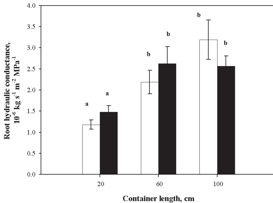
Figure 1. Root hydraulic conductance per leaf unit surface area ( K_{RL} , empty columns), and per root unit surface area ( K_{RR} , solid columns) for different container types. Average values accompanied by their standard error. Different letters denote significant differences ( p < 0.05 ), Tukey Test ( n = 10 ).
